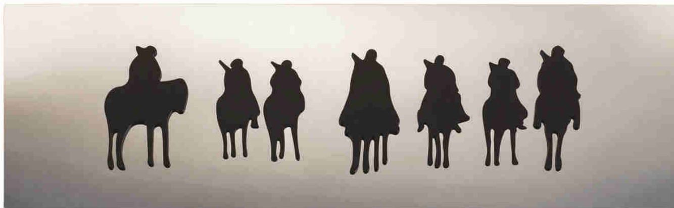
RUSSIAN ATMOSPHERE
